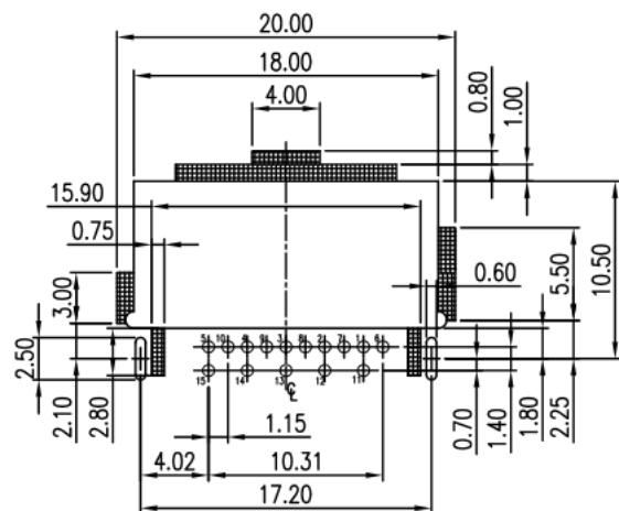
RECOMMENDED P.C.B LAYOUT (THICKNESS=1.00mm) GENERAL TOLERANCE±0.05mm
